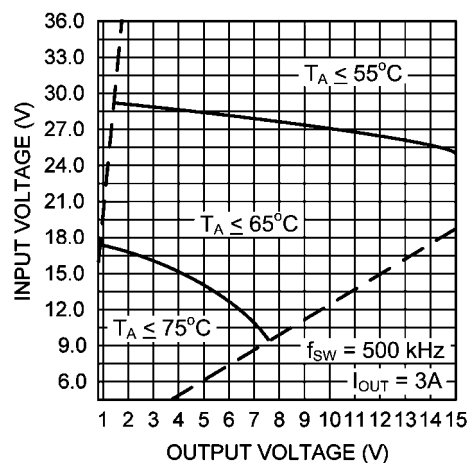
FIGURE 9. Safe Thermal Operating Areas ( I_{OUT} = 3A , f_{SW} = 500\text{kHz} )
